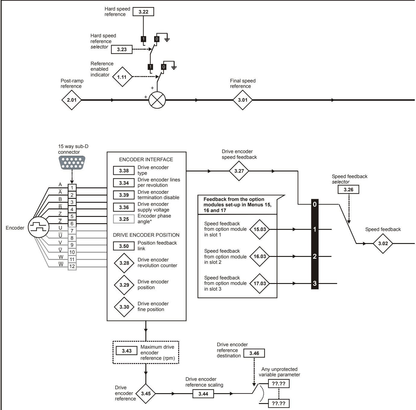
Figure 5-4 Menu 3 Closed-loop logic diagram
