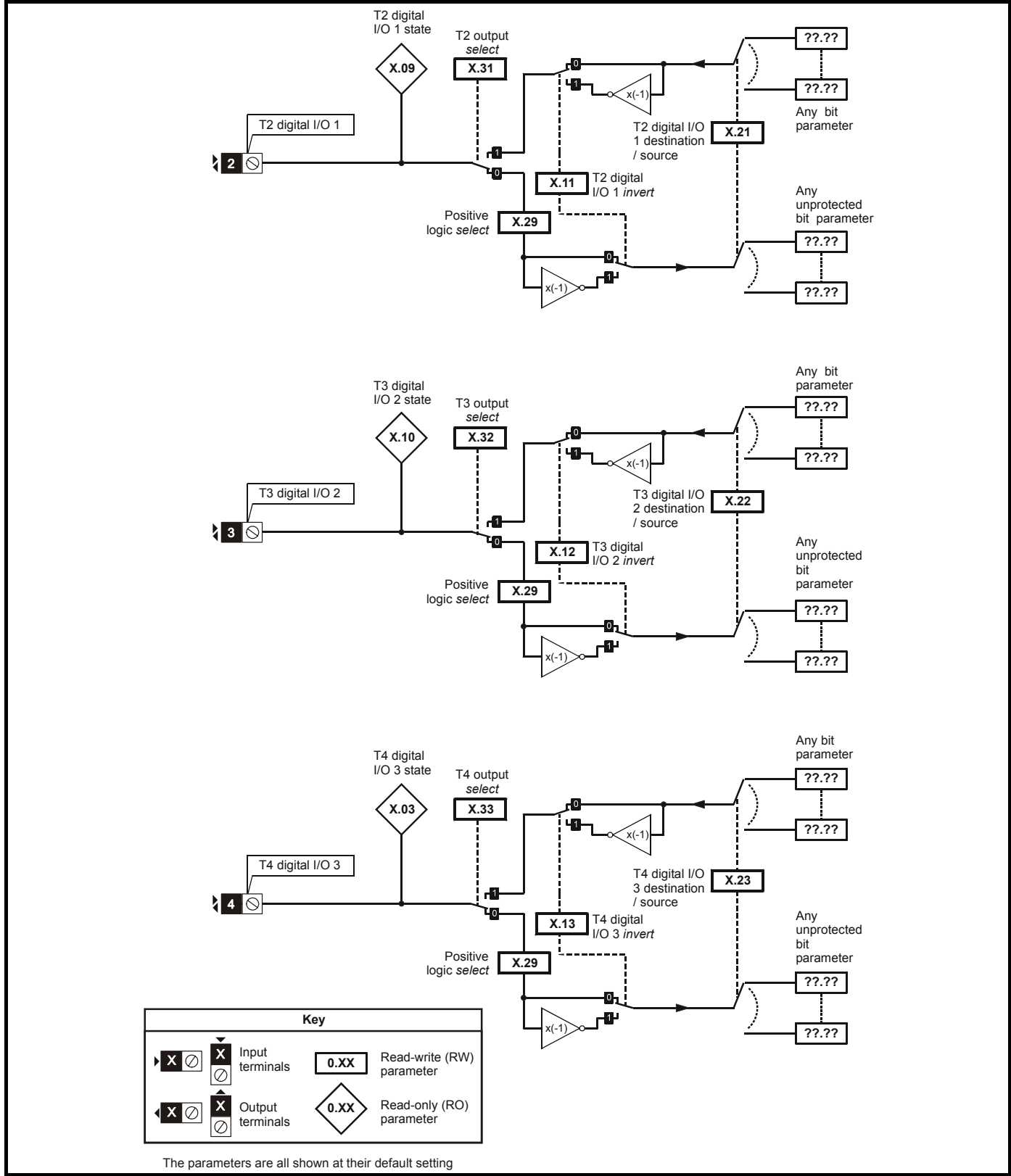
Figure 5-29 SM I/O Plus Digital Input/Output logic diagram 1
