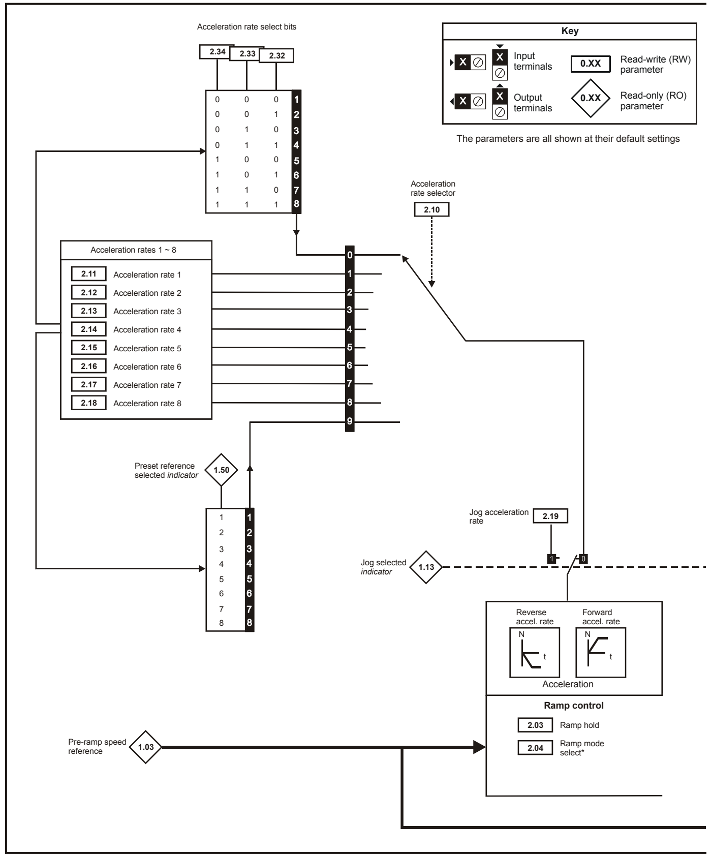
Figure 5-2 Menu 2 logic diagram
