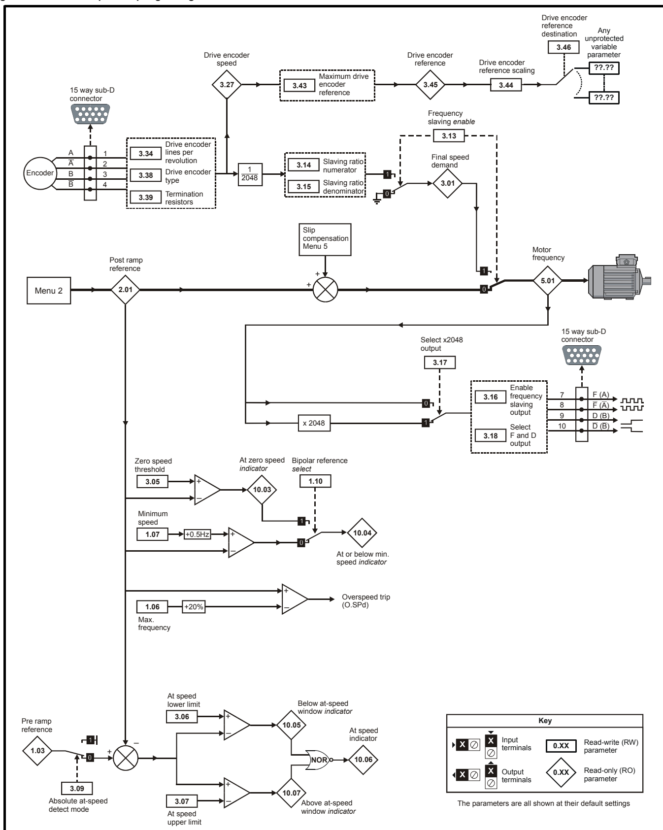
Figure 5-3 Menu 3 Open-loop logic diagram
