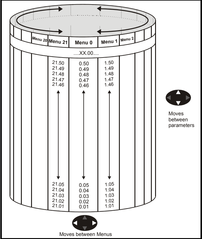
Figure 1-2 Menu structure
