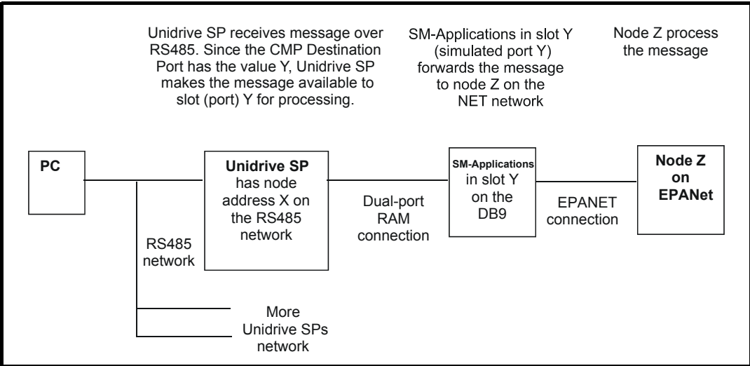
Figure 7-2 Example message routing from a PC through Unidrive SP and SM-Applications to a EPANet node
