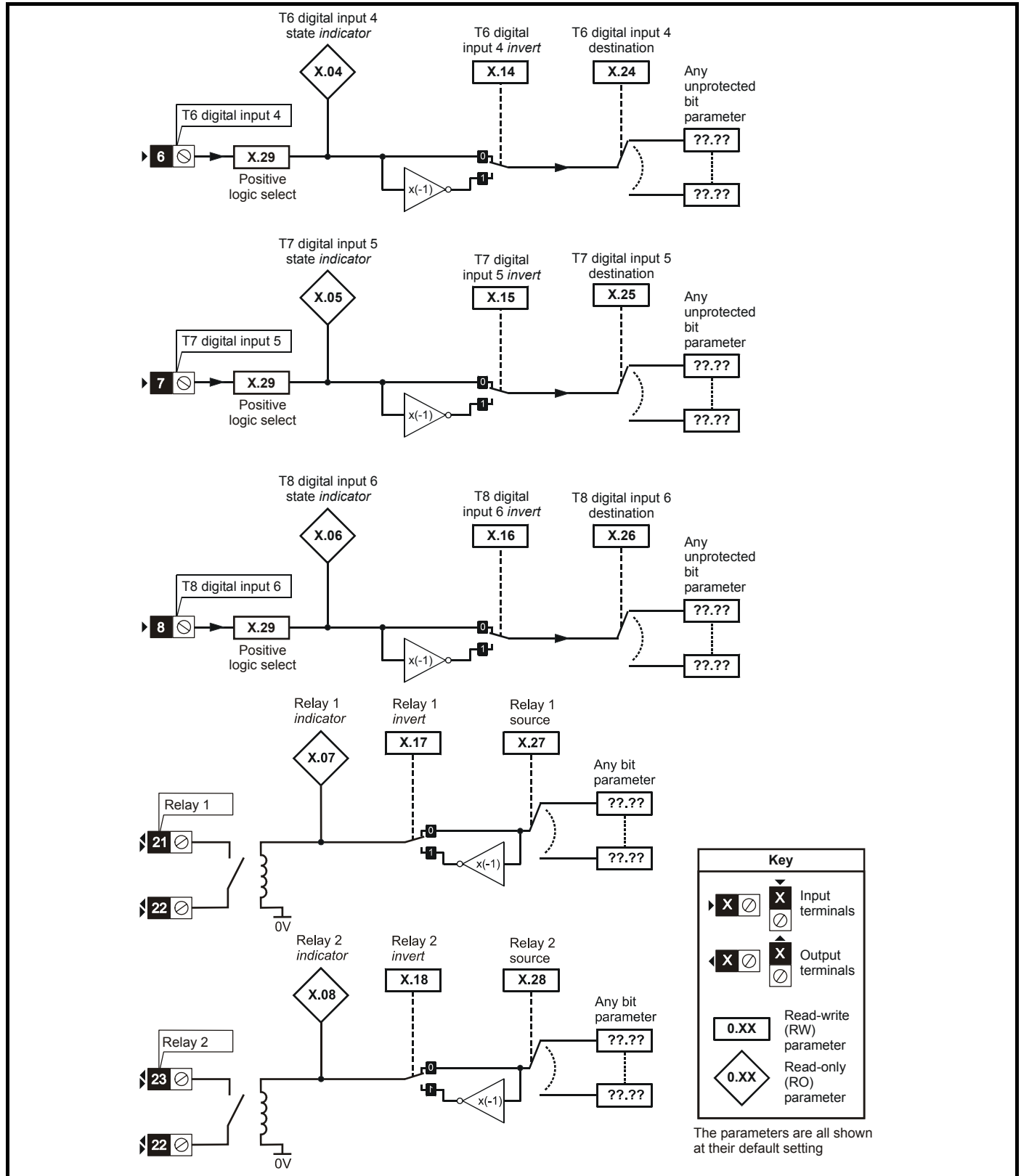
Figure 5-30 SM I/O Plus Digital Input/Output logic diagram 2
